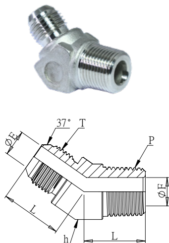
油壓 37° 45°彎外牙接頭 ( 精密鑄造 ) 45° Male Elbow( Investment Casting)
